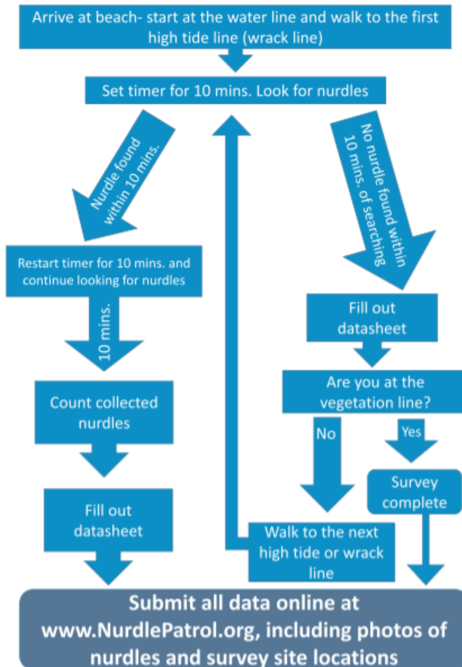
Fig. 2. Nurdle Patrol survey decision making flow chart.
